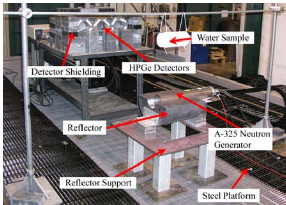
Figure 6. Experimental setup to measure the performance of the uranium reflector in reference to no reflector. The setup consisted of an MF-Physics A-325 D-T neutron generator, uranium reflector with support, HPGe detectors totaling 211% relative efficiency with digital processors and electromechanical coolers, lead detector shielding, and 2 liter high-density polyethylene bottle of water with support.
