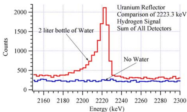
Figure 7. Comparison of hydrogen signal with and without 2-liter bottle of water for the uranium reflector. When the bottle is not present, there is no hydrogen signal in the background.
