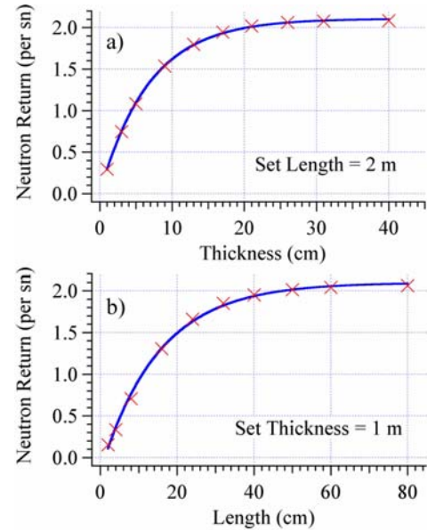
Figure 4. Neutron return for all energies across the top plane of the reflector as a function of the (a) thickness and (b) length. The optimal thickness (length) is 21 cm (46 cm) such that the neutron return is 95% of the maximum.
