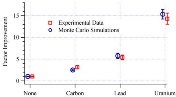
Figure 9. Improvement factor of uranium, lead, and carbon reflectors compared to no reflector. The uranium reflector enhances the hydrogen signal best, resulting in an enhancement of 15 over no reflector. The uranium enhancement is better than the next best material considered, lead, by a factor of at least 2.5.
