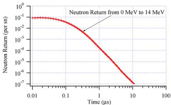
Figure 10. Neutron return through the top surface per source neutron entering the reflector at t=0 as a function of time after the neutron generator has been turned off. The return decreases at least 2 orders of magnitude after 1 \mu s, showing that the neutron flux from the reflector can be pulsed.
