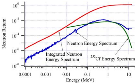
Figure 5. Neutron return as a function of energy across the top surface of the uranium reflector in the final design. The spectrum integration is also included. The neutron return maximizes at approximately 600 keV. The neutron return from 0 MeV to 14 MeV is 1.21 per source neutron entering the reflector.
