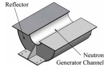
Figure 3. The uranium reflector.
