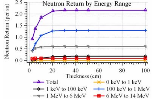
Figure 2. Plots of neutron return per source neutron entering the reflector as a function of thickness and of energy: a) 0 keV to 1 keV, b) 1 keV to 100 keV, c) 100 keV to 1 MeV, d) 1 MeV to 6 MeV, e) 6 MeV to 14 MeV, and f) the total energy range.
