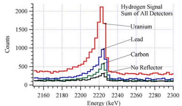
Figure 8. Hydrogen signal for the uranium, lead, carbon, and no reflectors.
