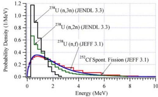
Figure 1. Emitted neutron energy spectrum for ^{238}\text{U} from neutron induced fission and ^{252}\text{Cf} from spontaneous fission. The spectra are very similar with peak energy near 1 MeV and average energy near 2 MeV.
